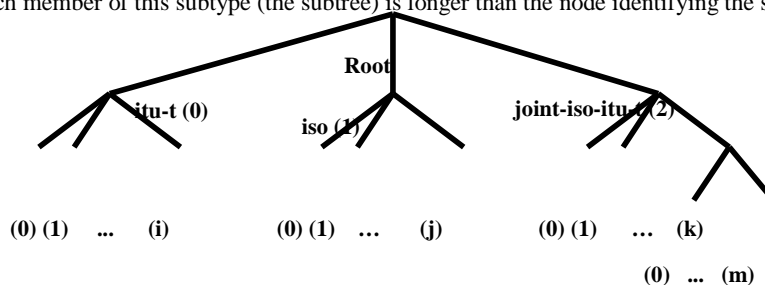
Figure 2: The object identifier tree
