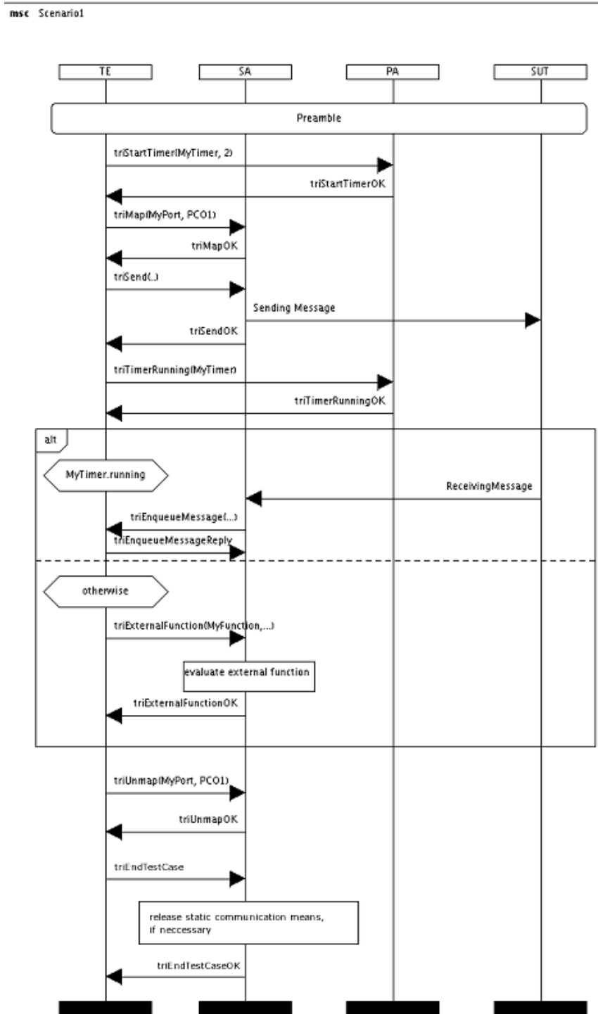
Figure B.2: Use Scenario 1
