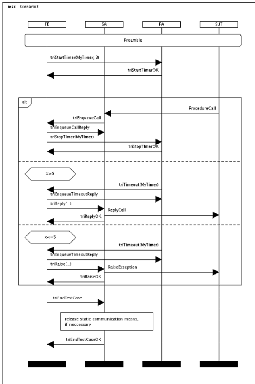
Figure B.4: Use Scenario 3
