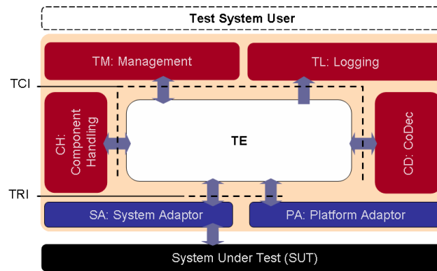
Figure 1: General Structure of a TTCN-3 Test System
