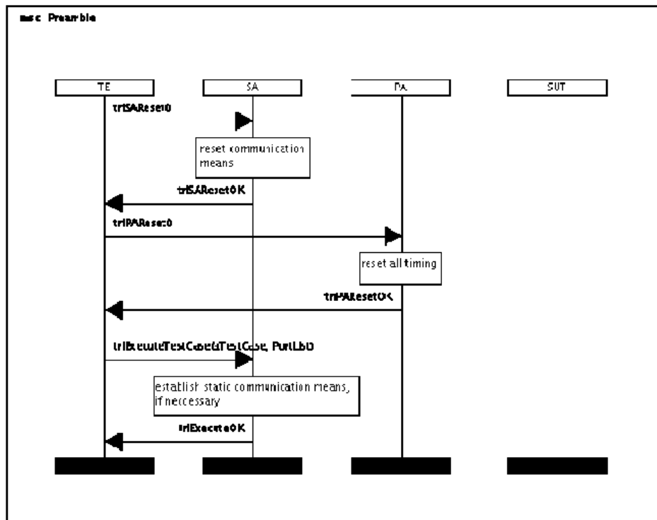
Figure B.1: Common MSC Preamble
