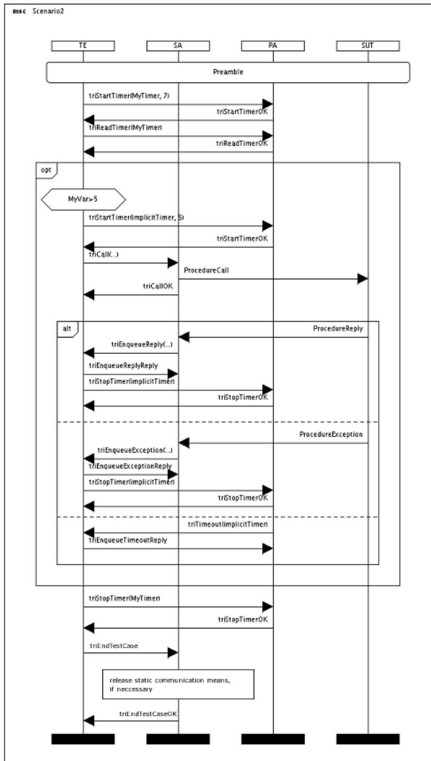
Figure B.3: Use Scenario 2
